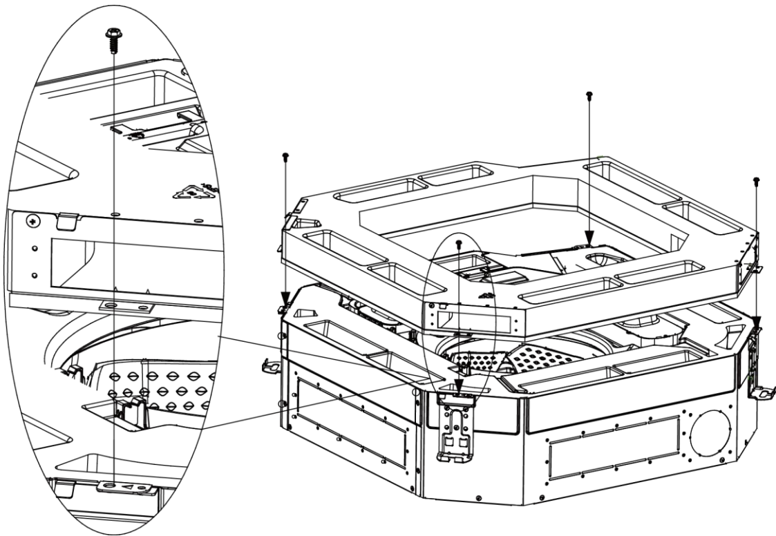
Install the main body
