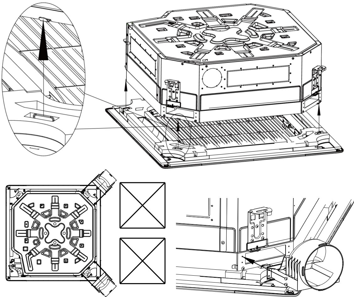
Install the front panel and fresh air opening
